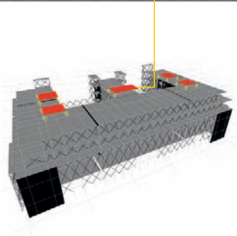
Model of Palatul Victoria with TMCS
